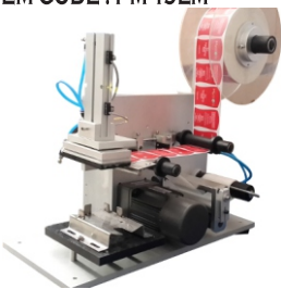
Semi Auto Flat Labeling Machine
