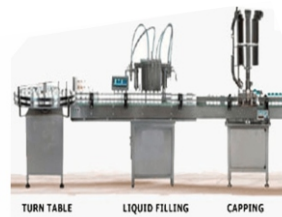
Fully Auto Liquid Filling With Capping Machine
