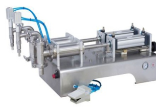
Two Heads Liquid Filling Machine
